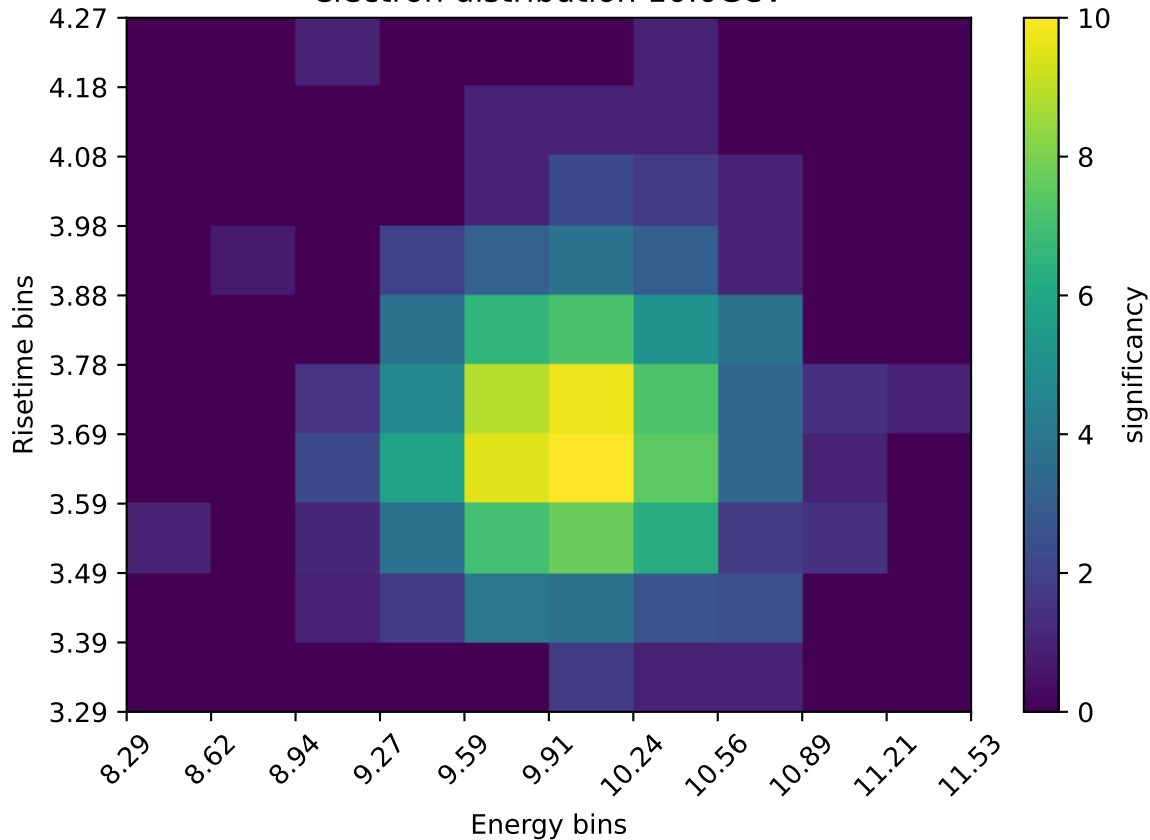
electron distribution 10.0GeV
